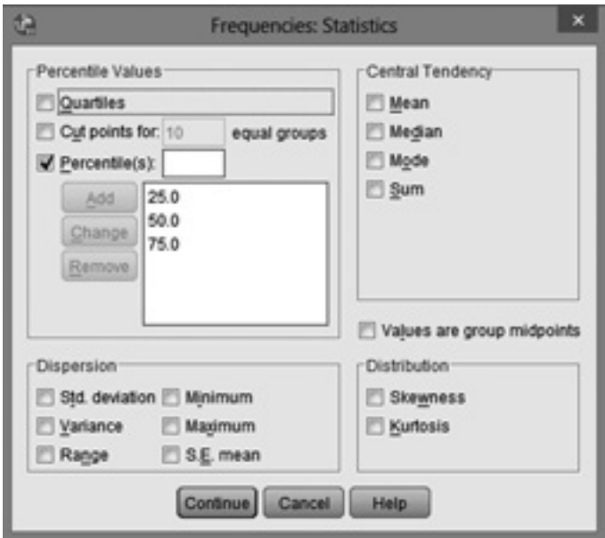
FIGURE 9.12 Computing percentiles
