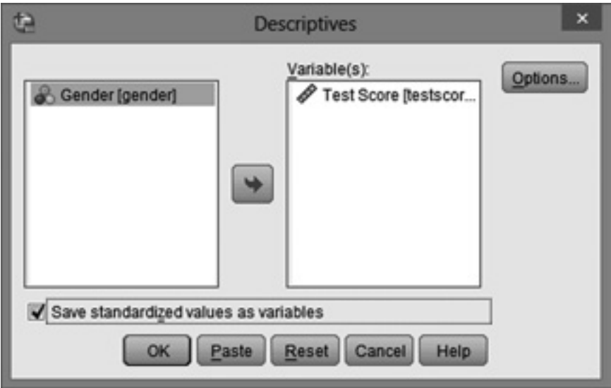
FIGURE 9.13 Generating z-scores
