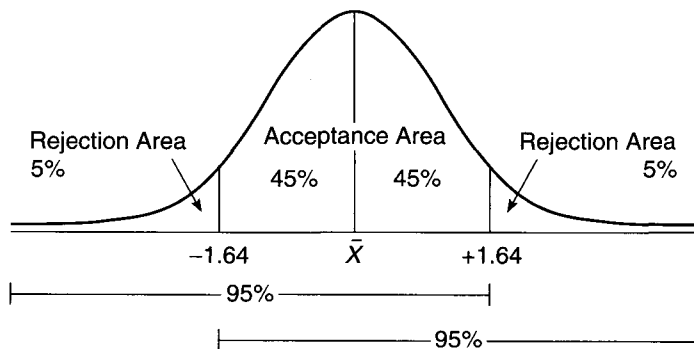
FIGURE 11.4 A One-Tailed Test at the .05 Level (5% at One End or 5% at the Other End)
