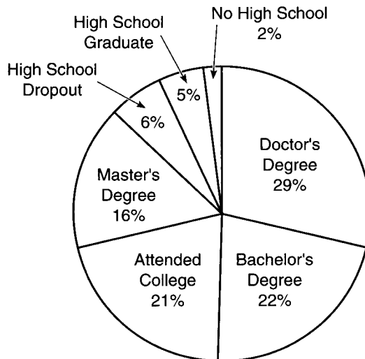
FIGURE 3.7 Educational Backgrounds of 129 American Celebrities Listed in the Current Biography 1966 Yearbook
