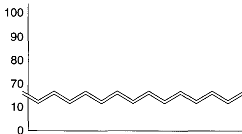
FIGURE 3.3 A Line Graph
