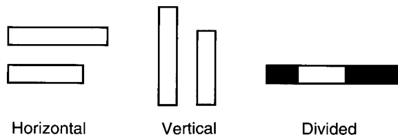
FIGURE 3.6 Divided Bars for Graphs
