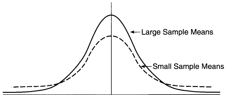
FIGURE 11.5 Distribution of Large and Small Sample Means
