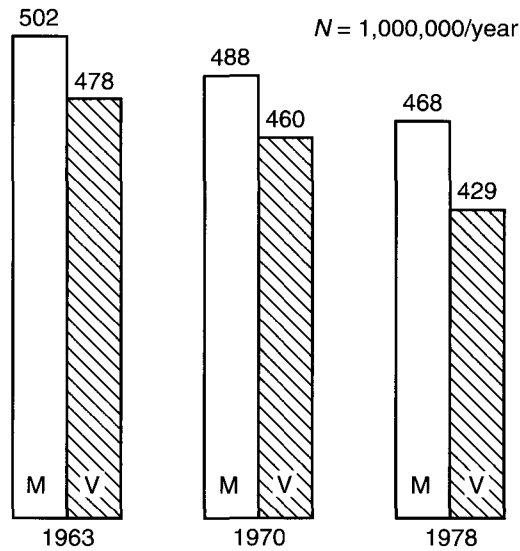
FIGURE 3.5 Decline of Mean Scholastic Aptitude Test Scores from 1963 to 1978
