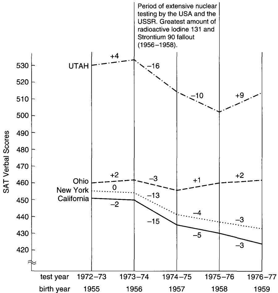
FIGURE 3.4 Mean Verbal SAT Scores, 1972–1977, in Four Selected States
