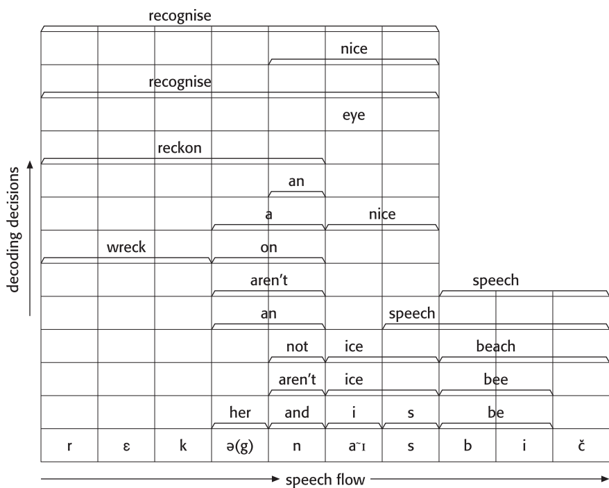
Figure 5.2 Decoding words and phrases during speech recognition. Speech recognition involves activating multiple candidates for words and phrases as the signal is being parsed. Here the incoming signal is ‘recognising speech’. Multiple candidate words and phrases are activated until the best candidate is decided
