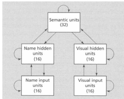
Functional architecture of Tippett and Farah's model of naming in Alzheimer's disease. The numbers refer to the number of units.
